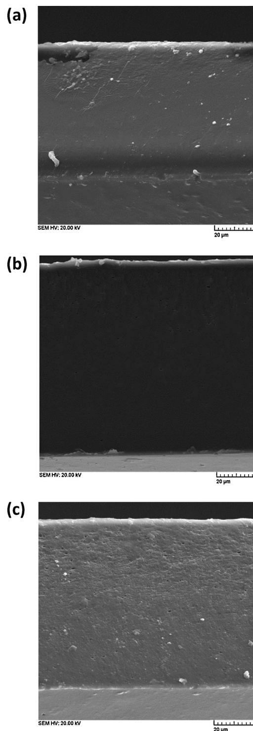
Fig. 6. Scanning electron microscopic images of cross-section of corn starch films: (a) control, (b) corn starch with 2% (v/v) ZEO and (c) corn starch with 2% (v/v) MEO.
